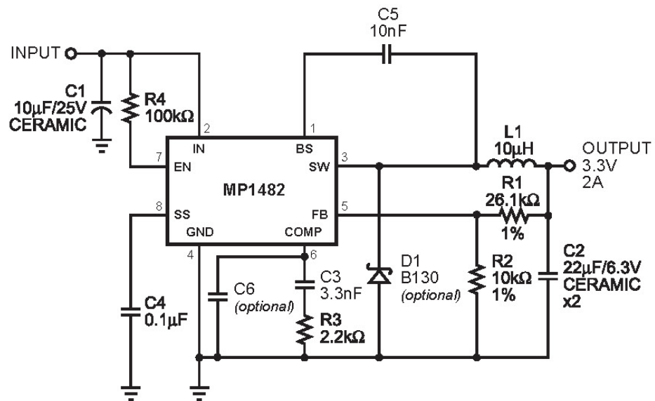
Figure 3—MP1482 with 3.3V Output, 22 \mu F/6.3V Ceramic Output Capacitor
